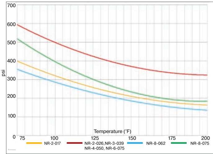
Nylon Tubing (Series NR) Maximum Working Pressure (psi)
